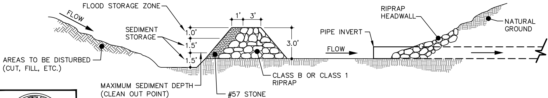
CROSS-SECTION VIEW
