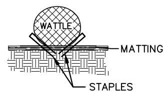
STAPLE INSTALLMENT SECTIONS
