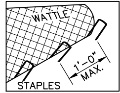
STAPLE INSTALLMENT SECTIONS
