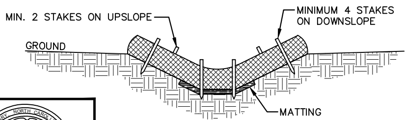
TRAPEZOIDAL DITCH SECTION VIEW
