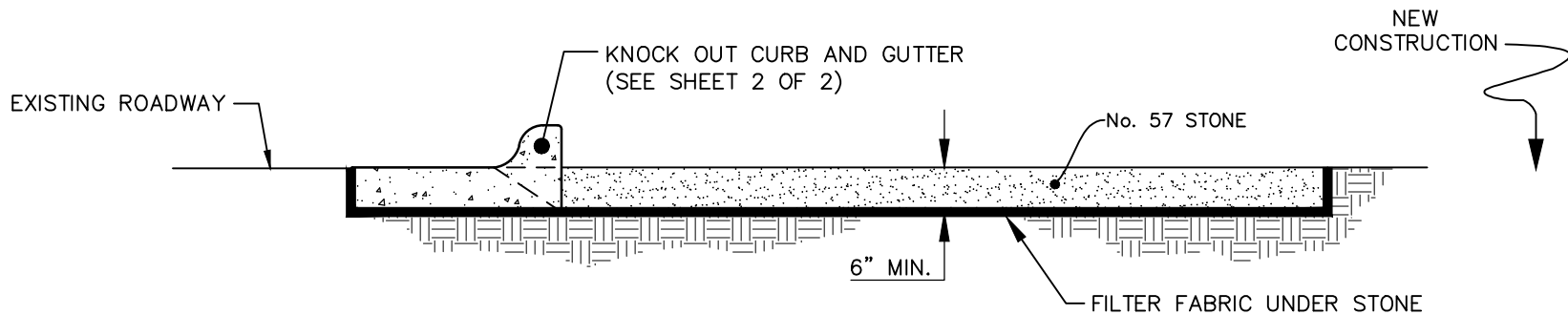
CROSS SECTION
