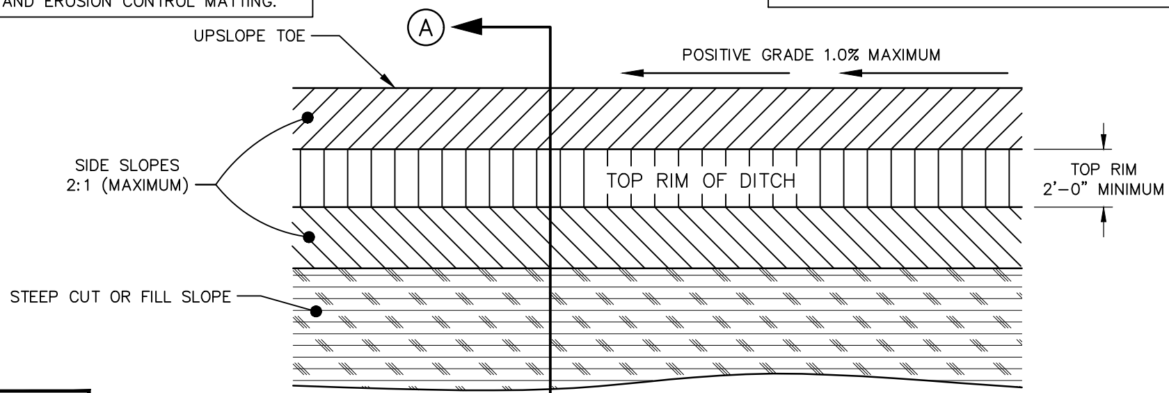
PLAN VIEW
