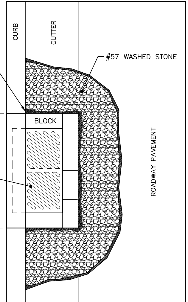
PLAN VIEW
