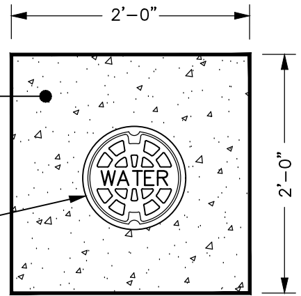
PLAN VIEW FOR UNPAVED AREAS
