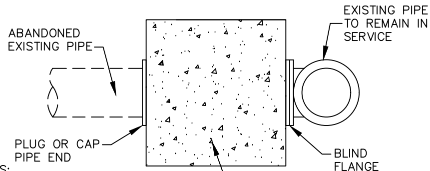
B. TYPICAL IN-LINE PIPE CUT AND RESTRAINED PLUG
