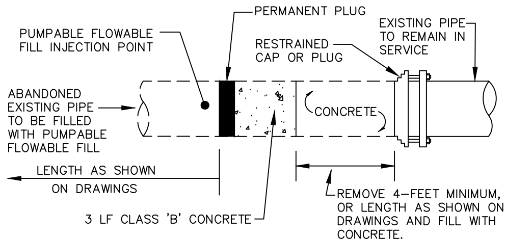
B. TYPICAL IN-LINE PIPE CUT AND RESTRAINED PLUG
