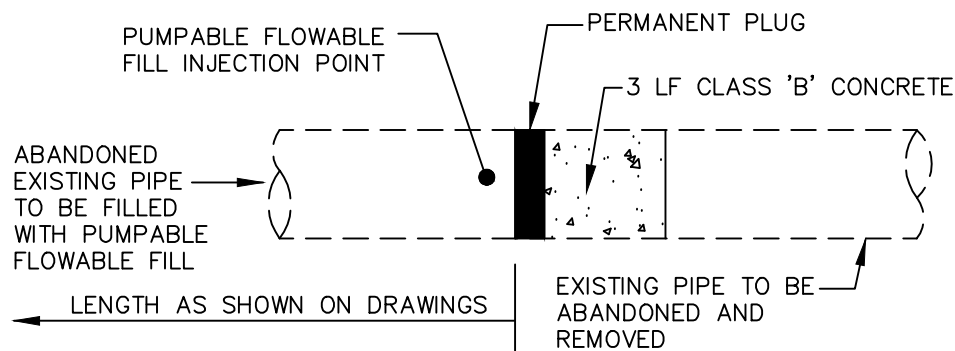
A. TYPICAL CUT AND PLUG
