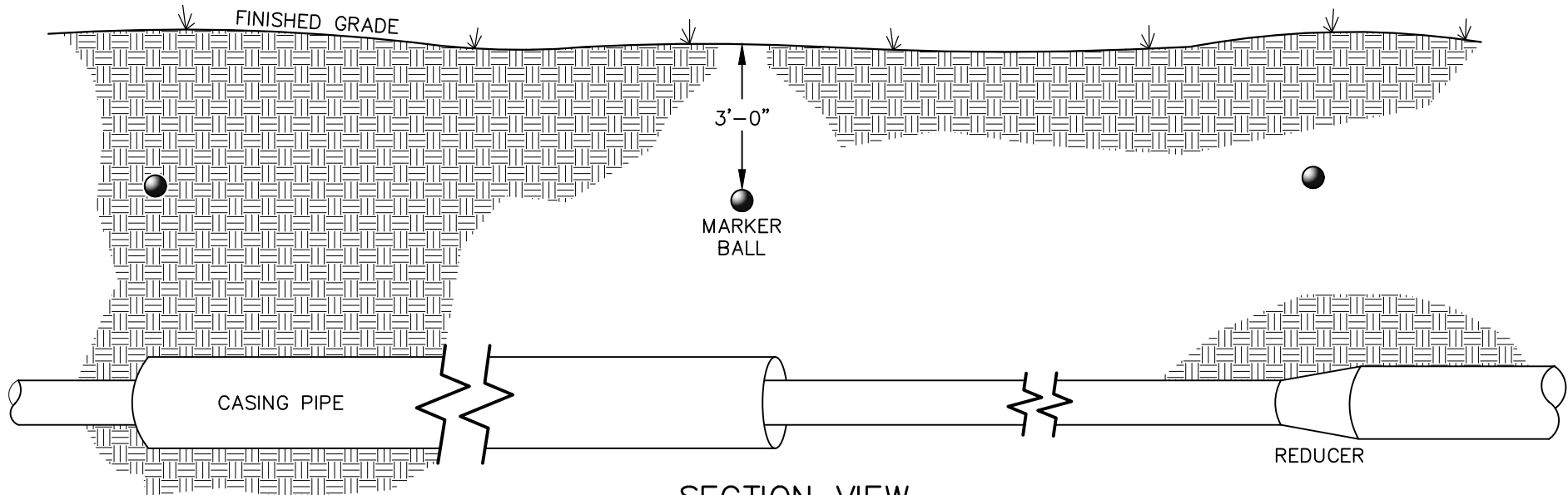
SECTION VIEW
