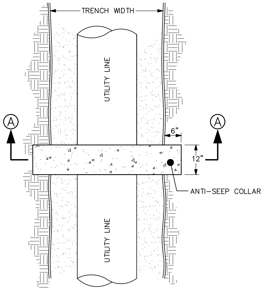
PLAN VIEW
