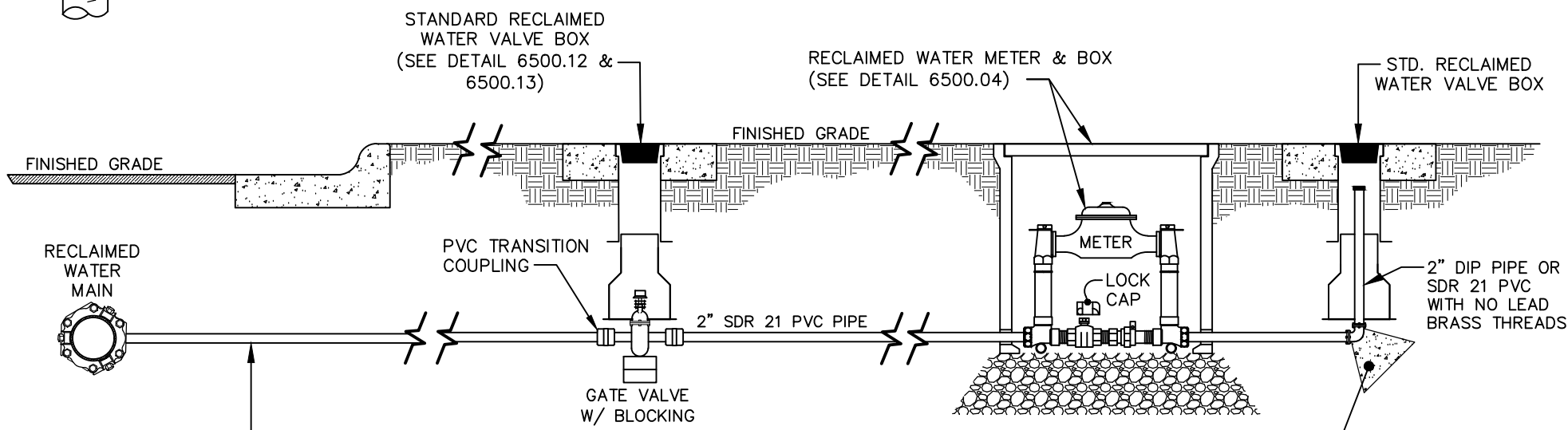
SECTION VIEW
