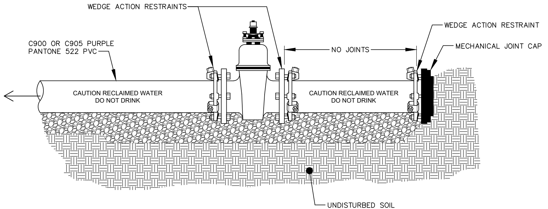
SECTION VIEW
