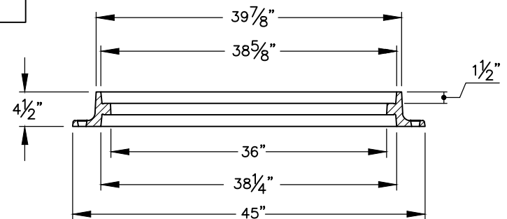
FRAME SECTION
