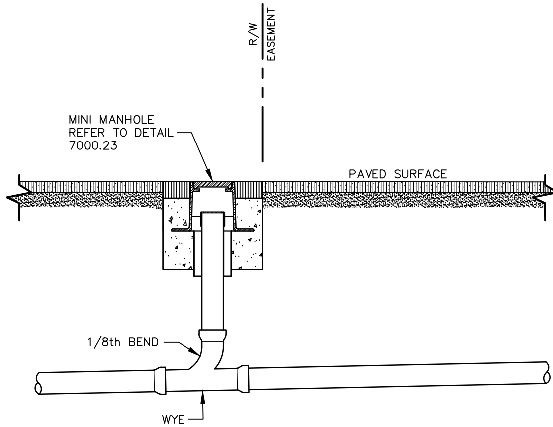
SECTION VIEW
