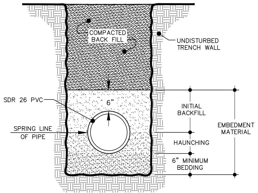
SPECIAL BEDDING FOR 14'-20' DEPTHS
