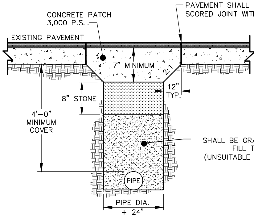
CONCRETE PAVEMENT
