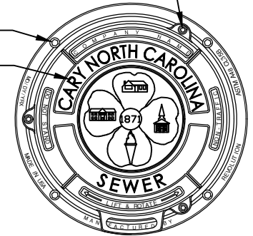
RING & COVER TOP VIEW
