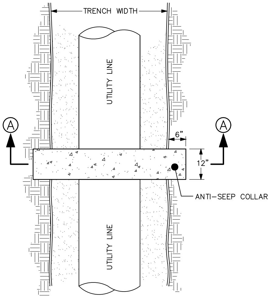
PLAN VIEW
