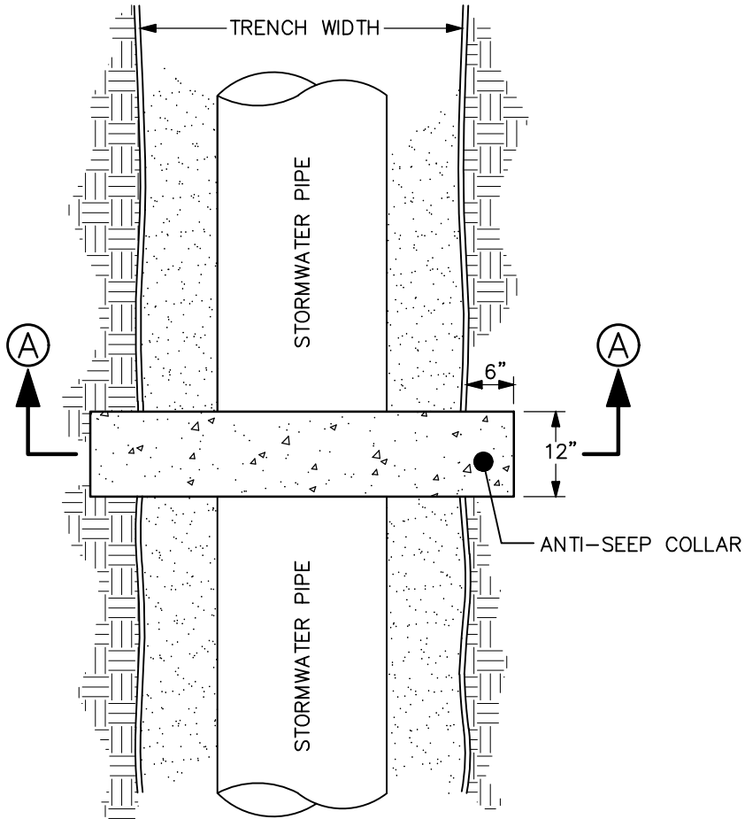
PLAN VIEW
