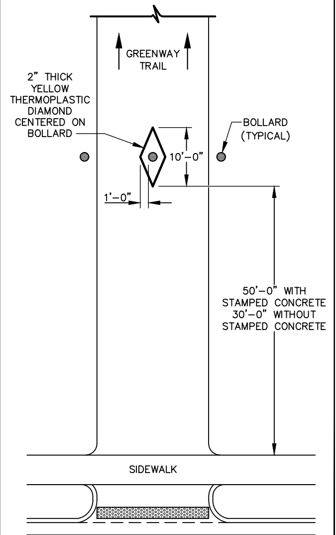
PLAN VIEW
