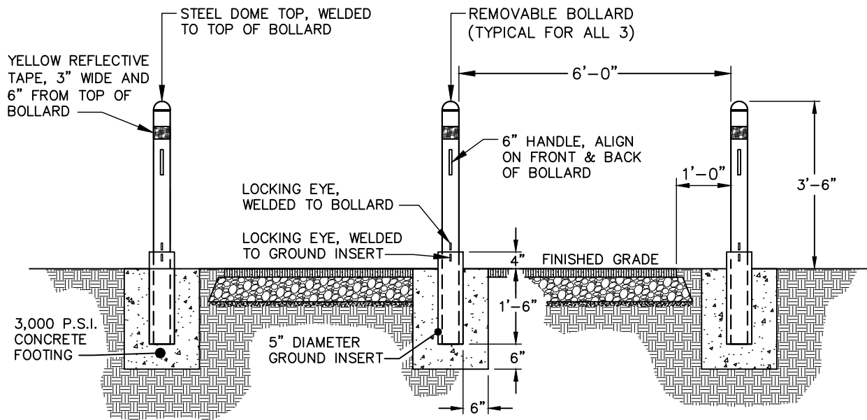
FRONT VIEW
