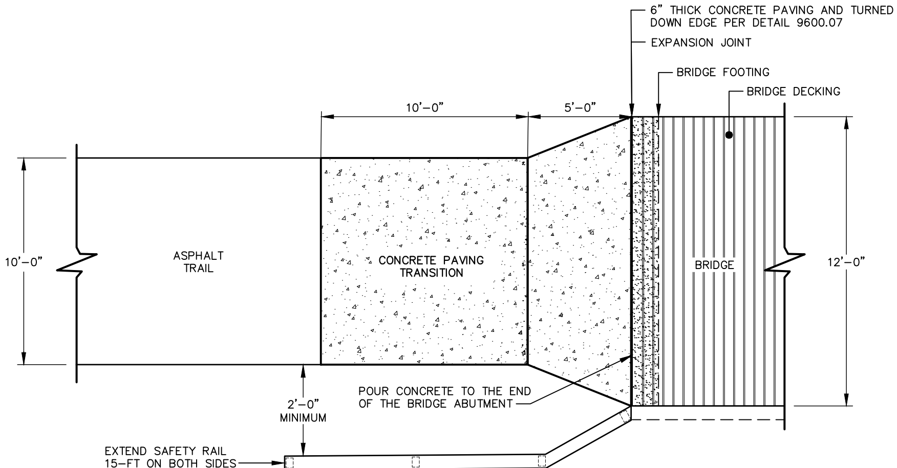
PLAN VIEW
