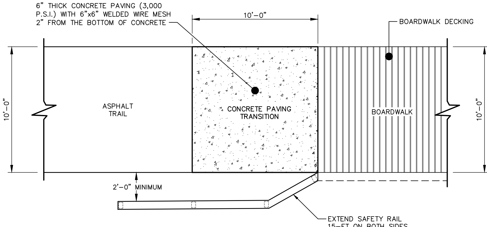
PLAN VIEW
