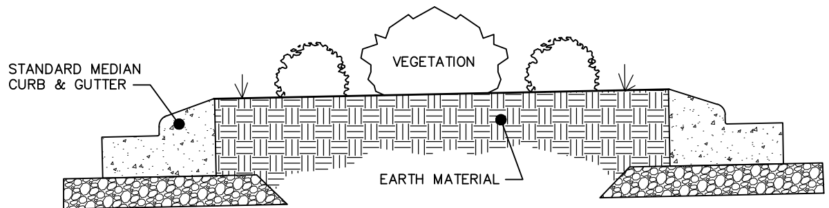
LANDSCAPED MEDIAN SECTION VIEW
