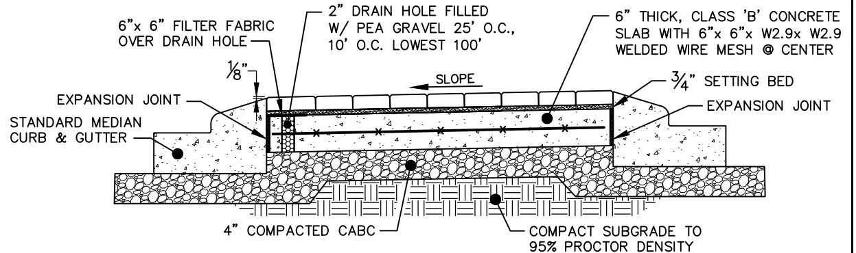
BRICK PAVER MEDIAN SECTION VIEW
