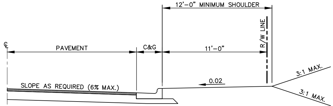
SECTION 'A-A' WITH CURB & GUTTER
