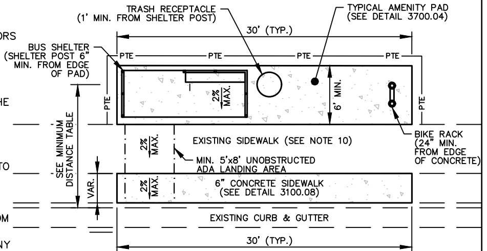
SHELTER WITH SIDEWALK AND UTILITY STRIP
