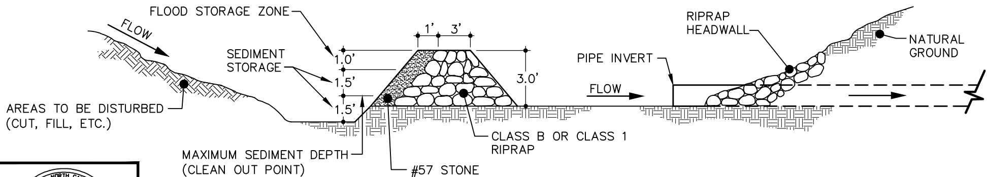
CROSS-SECTION VIEW
