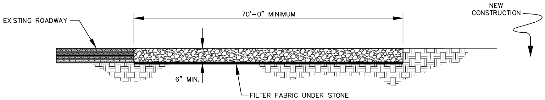
CROSS SECTION
