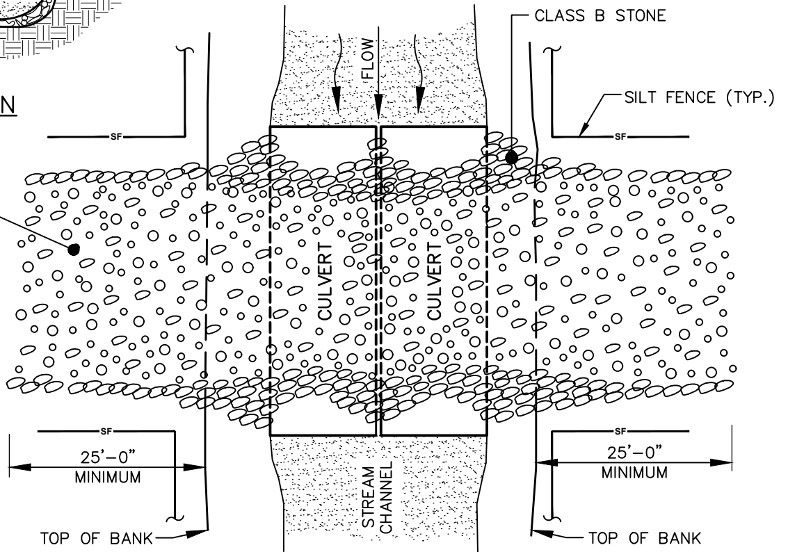
PLAN VIEW
