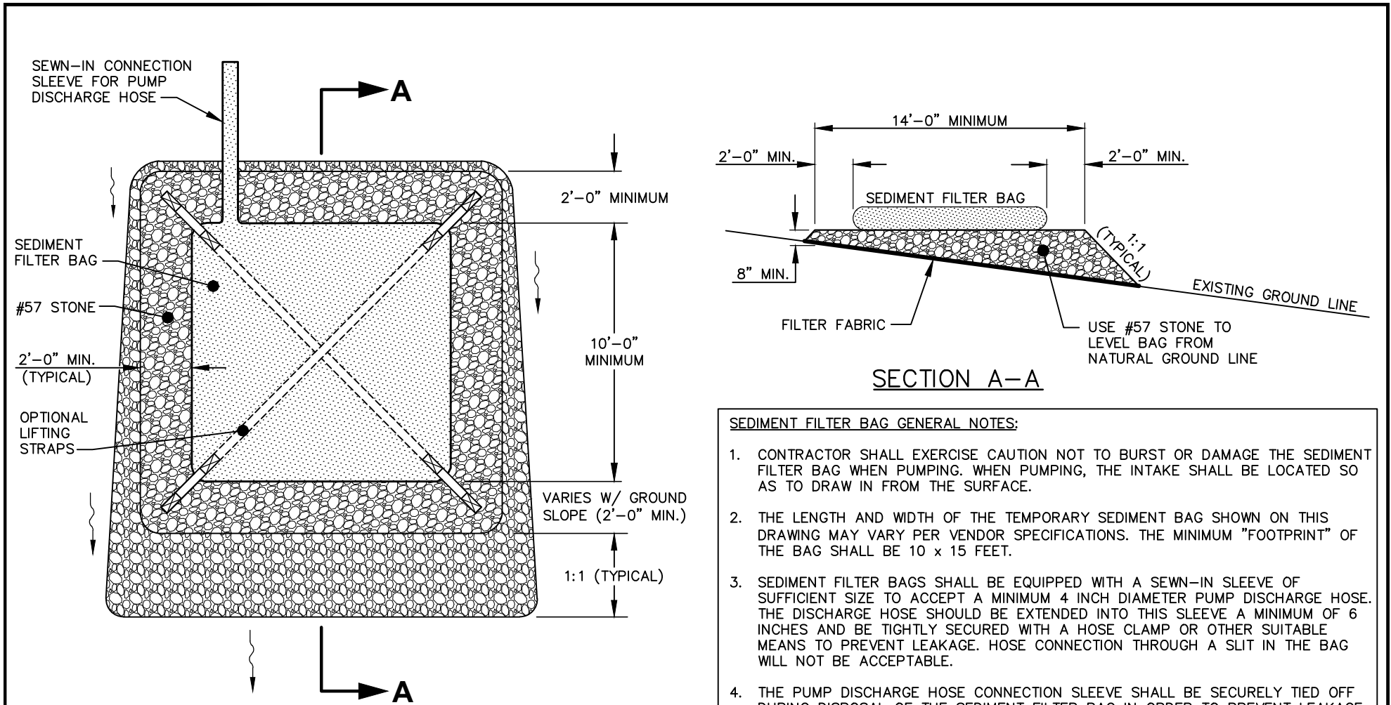
PLAN VIEW
