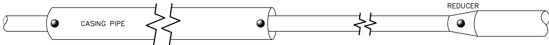
PLAN VIEW
