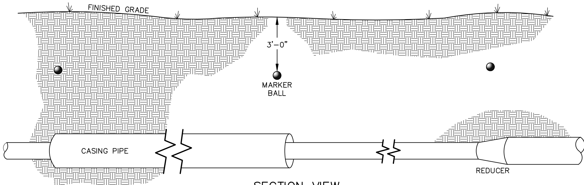
SECTION VIEW
