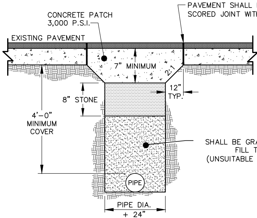
CONCRETE PAVEMENT
