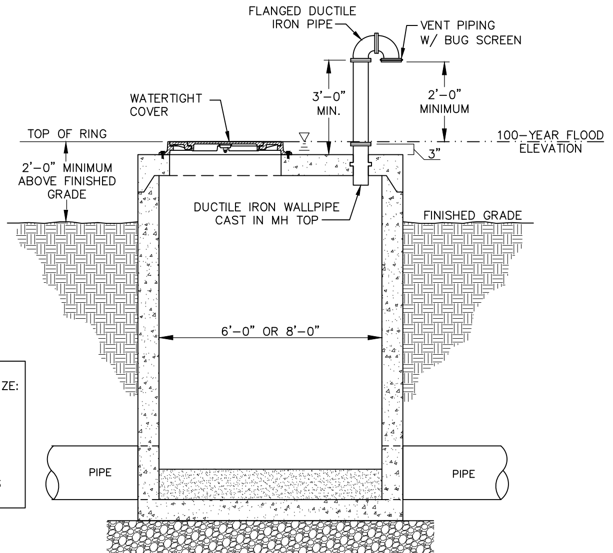
SECTION VIEW
