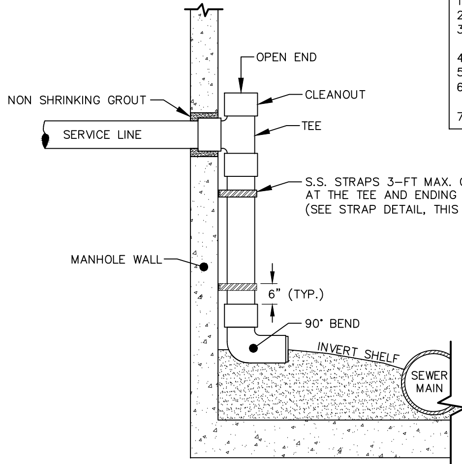
SECTION VIEW
