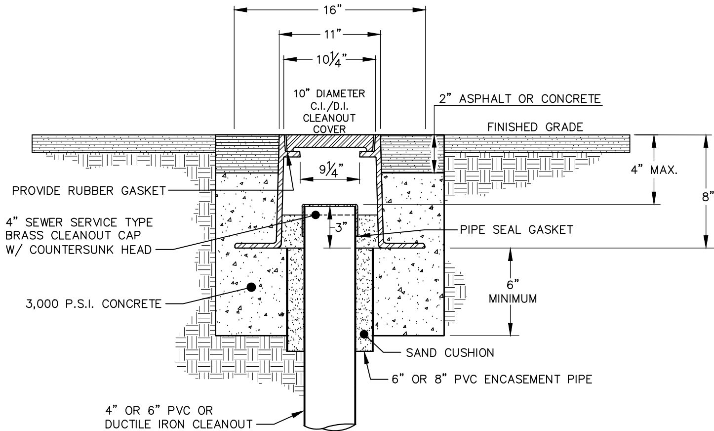
SECTION VIEW
