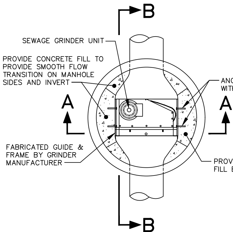
PLAN VIEW
