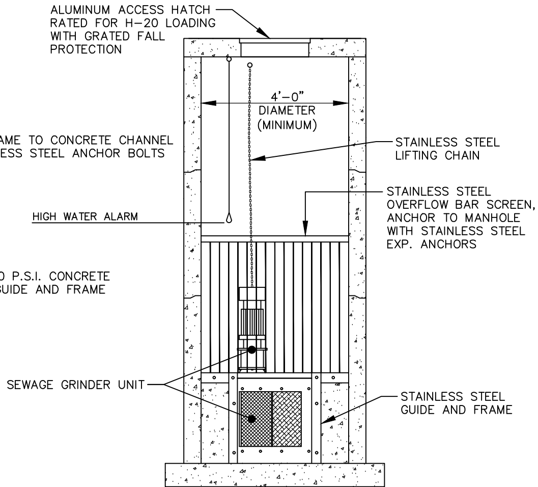
SECTION "A-A"
