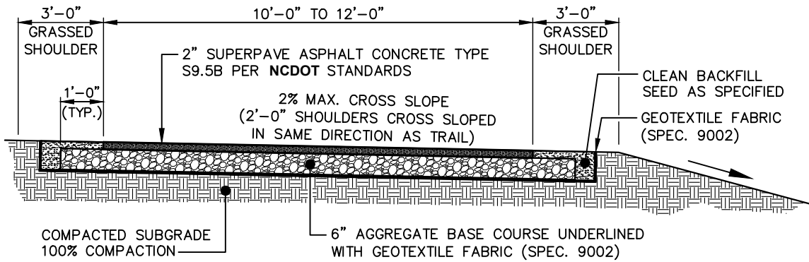
TYPICAL SECTION
