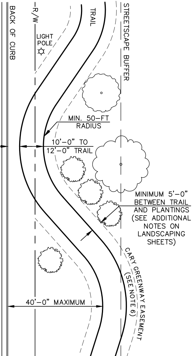
PLAN VIEW
