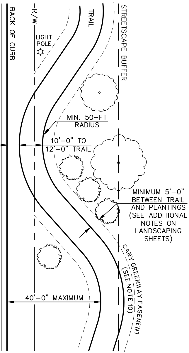
PLAN VIEW
