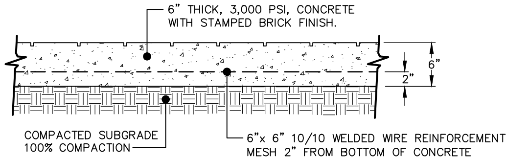
SECTION VIEW
