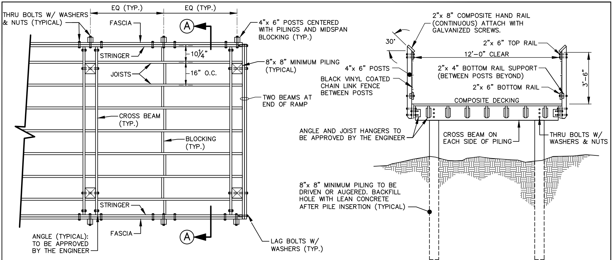
PLAN VIEW (FOR ELEVATION VIEW SEE DETAIL 9500.08)
