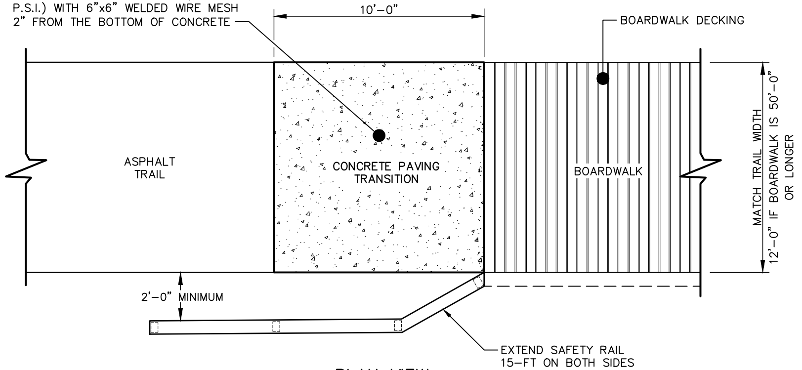
PLAN VIEW
