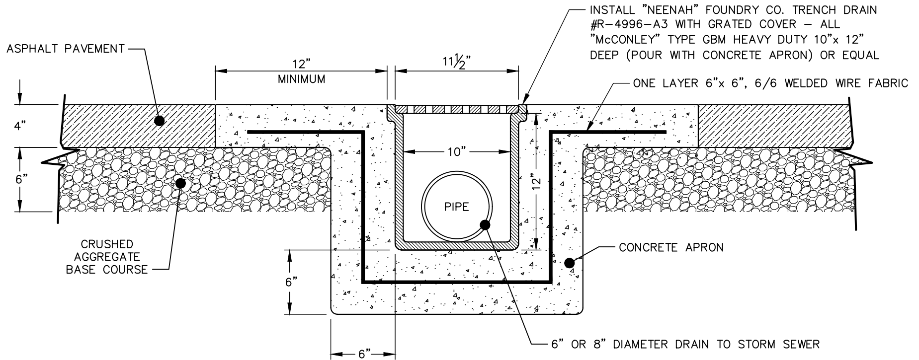
SECTION VIEW
