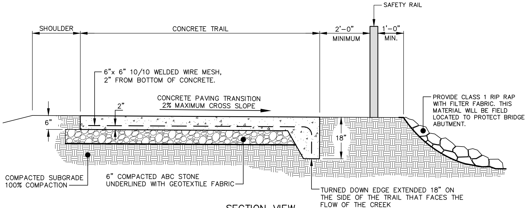
SECTION VIEW
