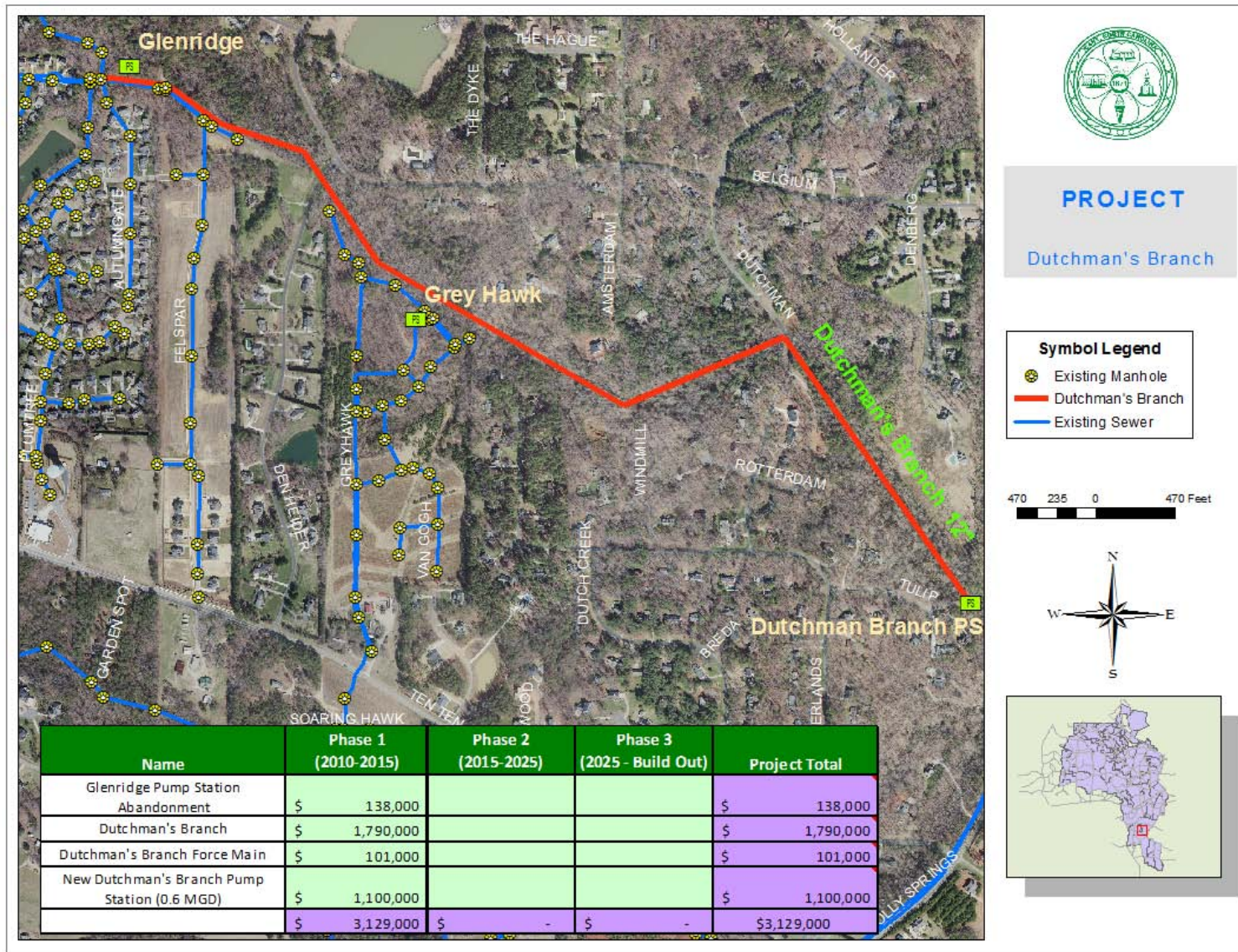
Figure 7-11: Dutchman's Branch Interceptor
