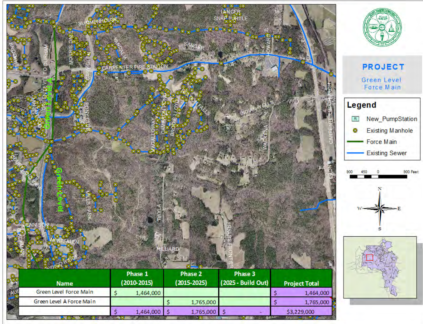
Figure 7-15: Details of Green Level Force Main
