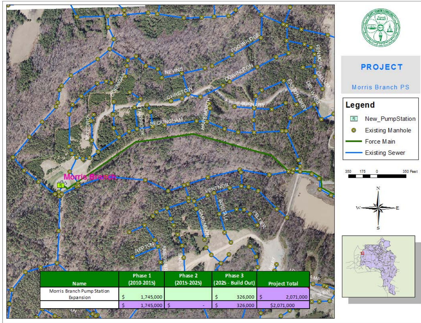
Figure 7-19: Morris Branch Pump Station Upgrade
