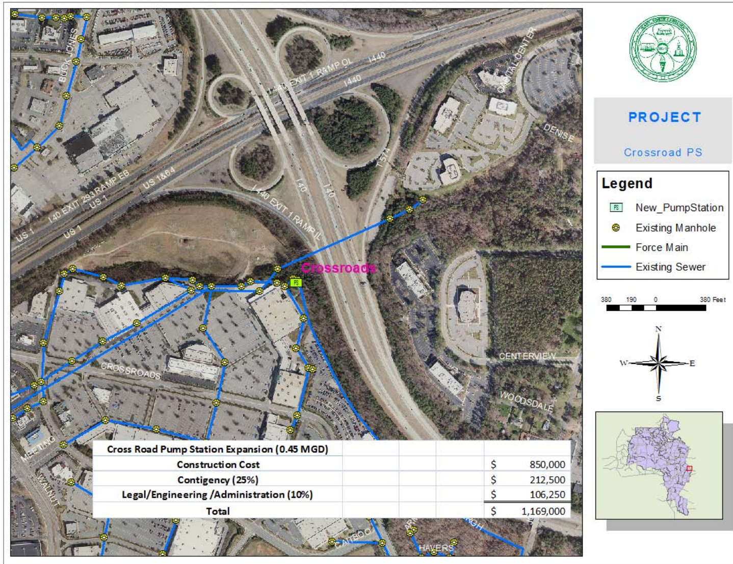
Figure 7-23: Cross Roads Pump Station Upgrade
