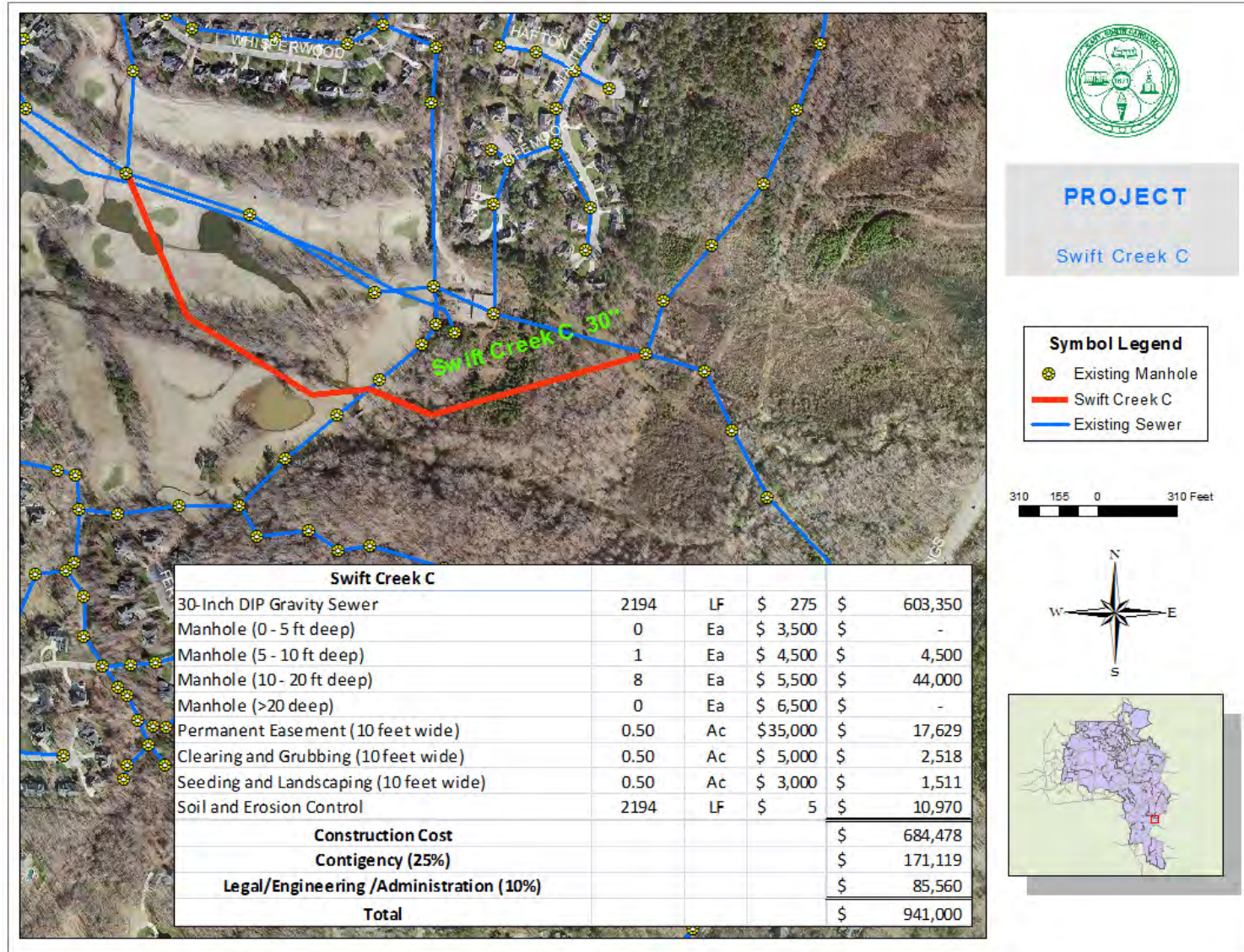
Figure 7-26: Swift Creek Interceptor C
