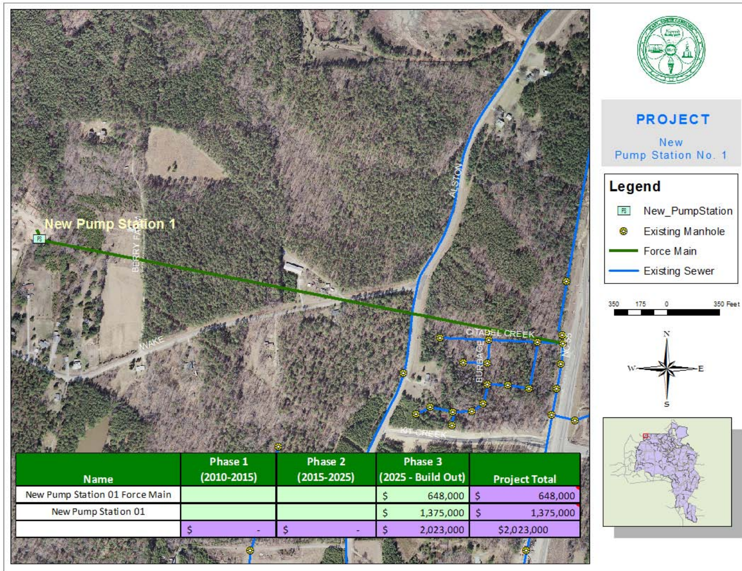
Figure 7-33: Pump Station No. 1 and Force Main
