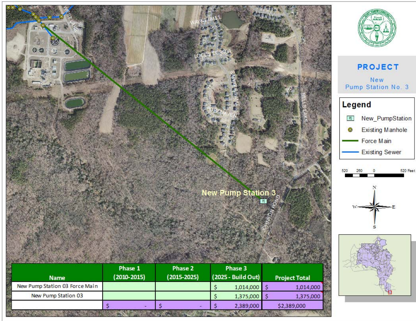
Figure 7-35: New Pump Station No. 3 and Force Main
